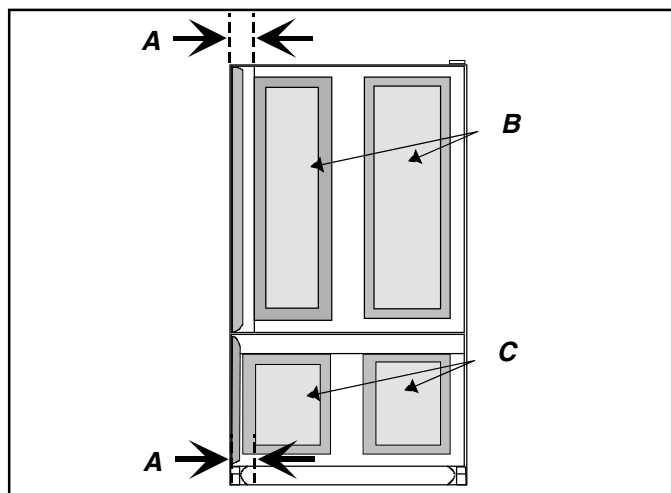
A 2 1/2" clearance from raised panel edge to edge of door. B Raised panel—41" x 35 5/8" (104 cm x 90.5 cm) C Raise panel—23 11/16" x 35 5/8" (60.2 cm x 90.5 cm)
