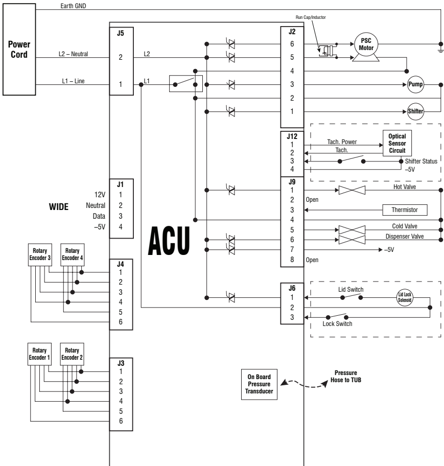
Figure 9 - Wiring Diagram
